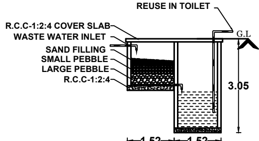
RECYCLING OF WASTE WATER BATH ROOM
