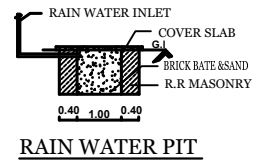
RAIN WATER PIT
