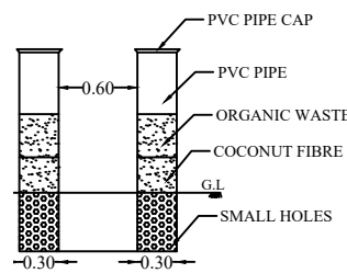
IPE COMPOSIT PIT
