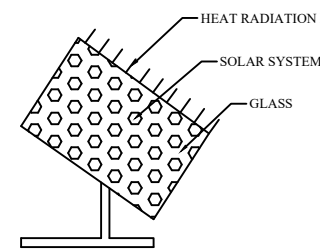
SOLAR SYSTEM
