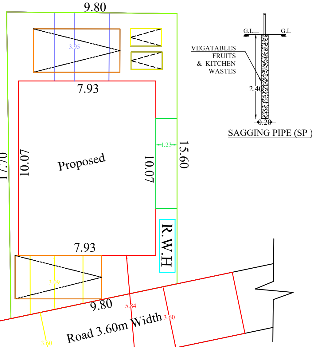
SITE PLAN
