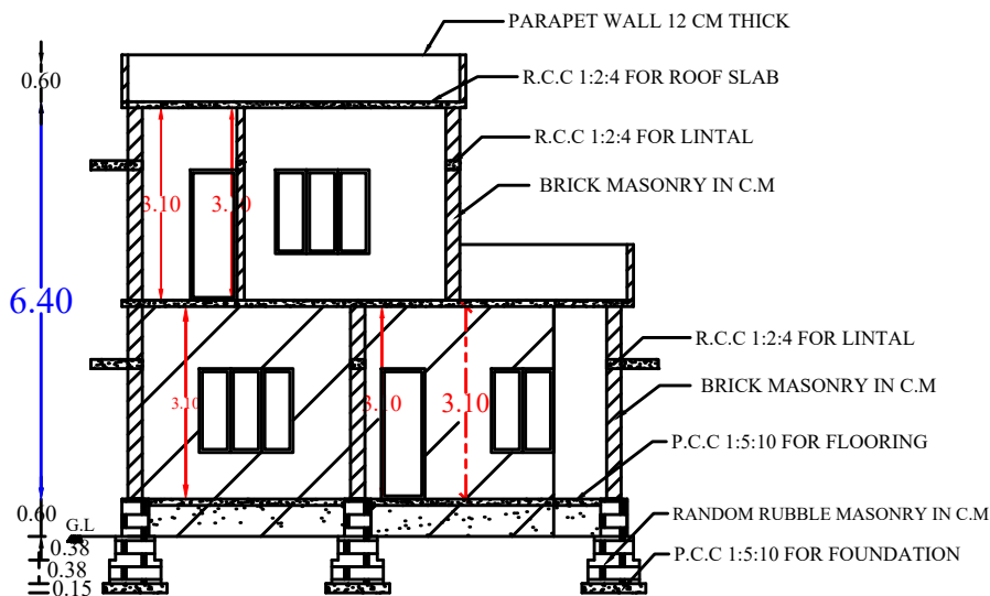
SECTION
