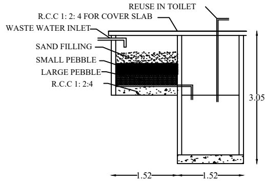
RECYCLING OF WASTE WATER
