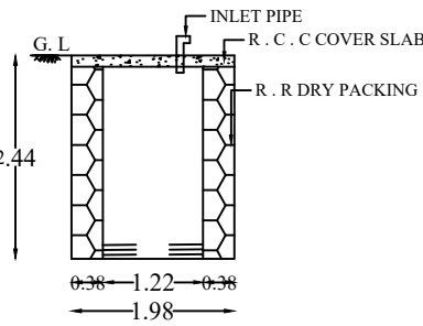
WATER STORAGE TANK SECTION
