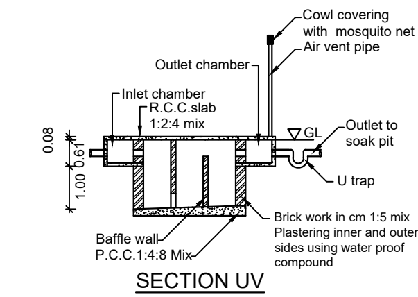
SECTION UV
