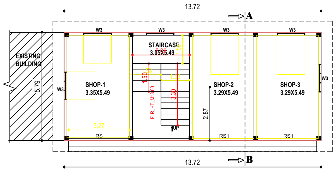
SCALE 1:100 ALL DIMENSIONS ARE IN METRE
