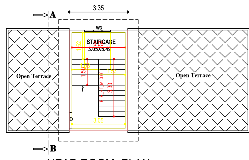
HEAD ROOM- PLAN
