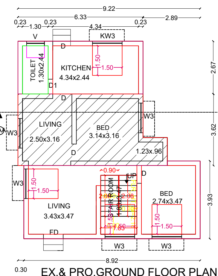
EX. & PRO.GROUND FLOOR PLAN
