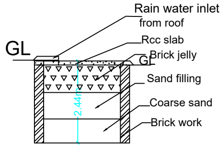
RAIN WATER HARVESTING PIT
