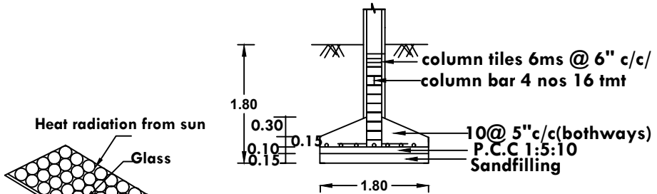
SECTION OF COLUMN
