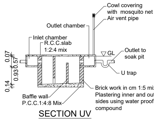
SECTION UV
