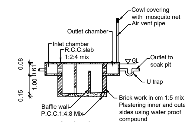
SECTION UV
