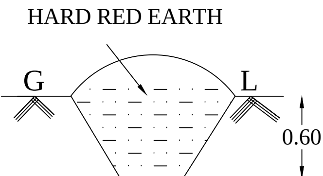
PIT SECTION
