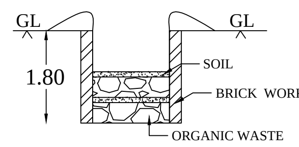
COMPOST PIT
