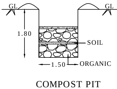
COMPOST PIT
