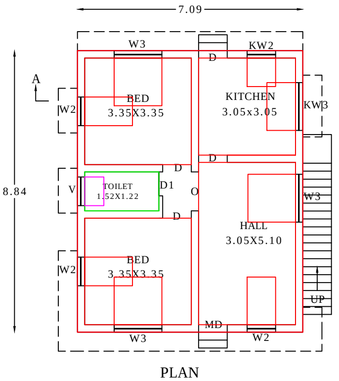
PLAN
