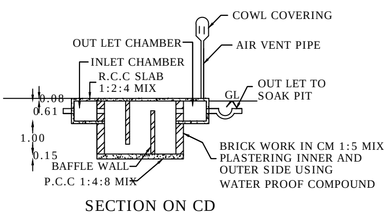
SECTION ON CD
