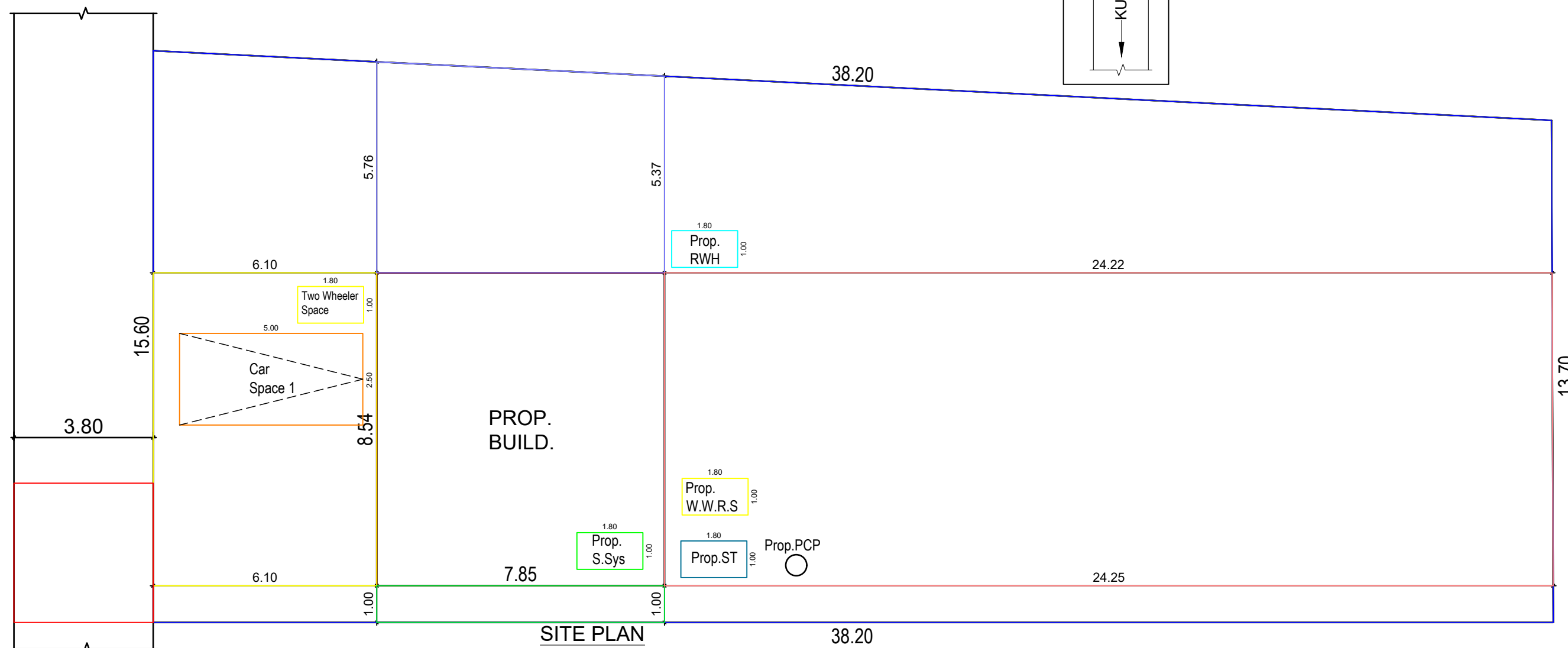
SITE PLAN
