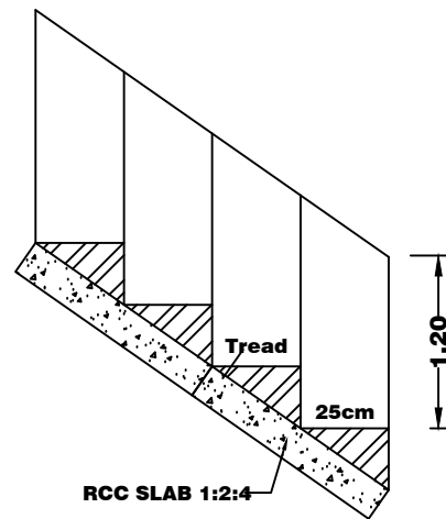
STAIR DETAILS
