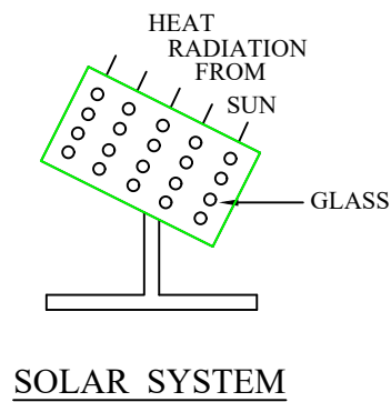
SOLAR SYSTEM
