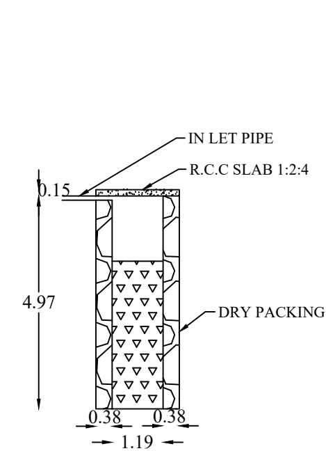
WASTE WATER TANK
