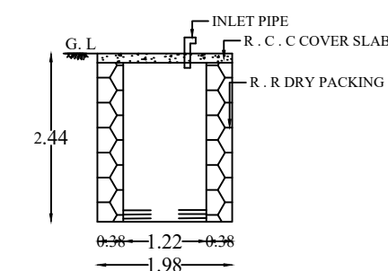
RAIN WATER STORAGE TANK SECTION
