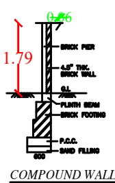
COMPOUND WALL DETAIL
