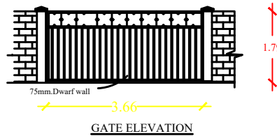
GATE ELEVATION
