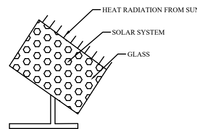
SOLAR SYSTEM
