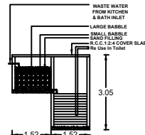
RECYCLING OF WASTE WATER FROM KITCHEN & BATHROOM (Scale 1:100)
