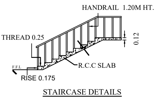
STAIRCASE DETAILS
