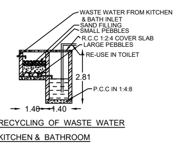
RECYCLING OF WASTE WATER KITCHEN & BATHROOM
