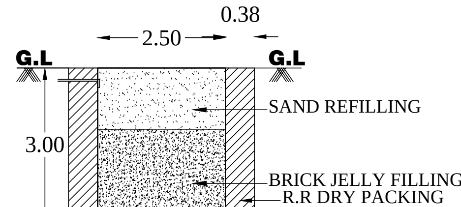
RAINWATER HARVESTING
