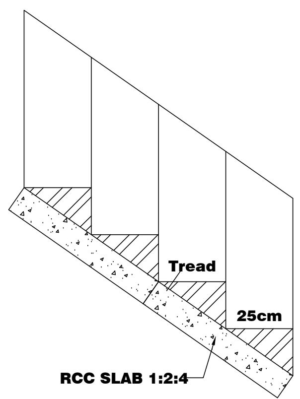
STAIR DETAILS
