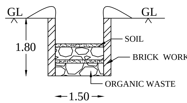
COMPOST PIT
