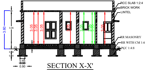
SECTION X-X'
