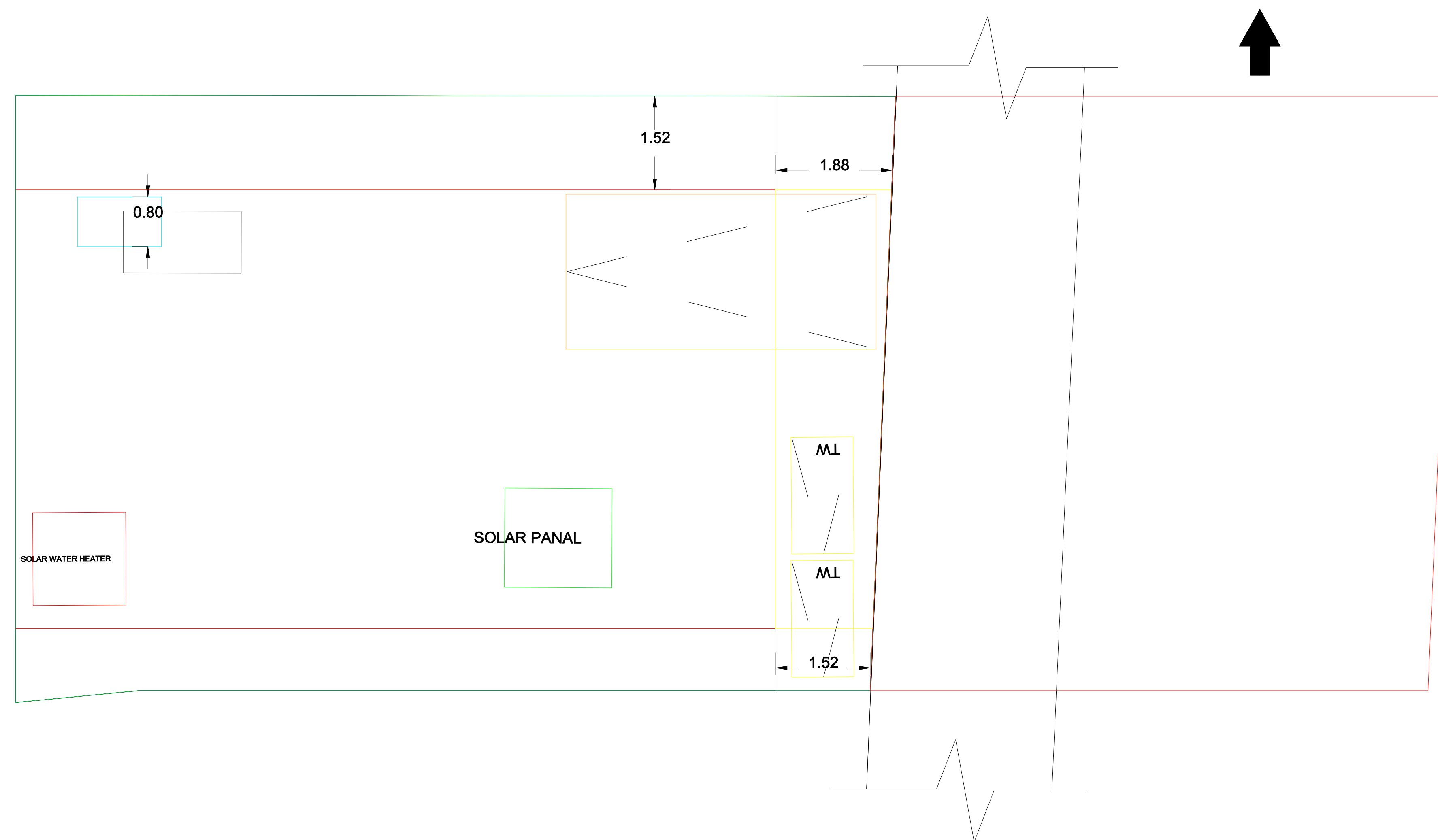
SITE PLAN
