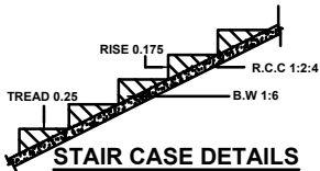
STAIR CASE DETAILS
