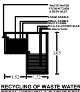
RECYCLING OF WASTE WATER FROM KITCHEN & BATHROOM
