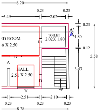
IRST FLOOR
