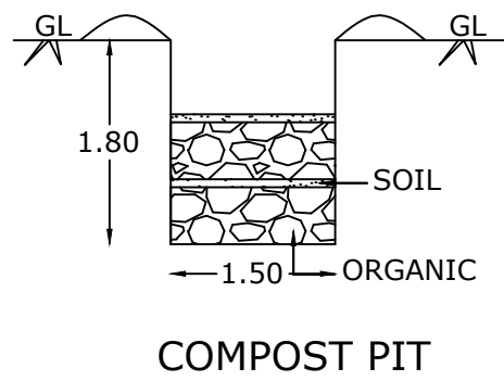
COMPOST PIT
