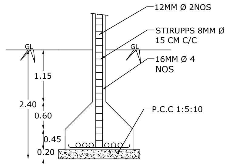
COLUMN DETAILS (SIZE 0.23X0.23) SCALE 1:50
