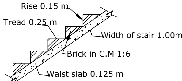
STAIR DETAILS
