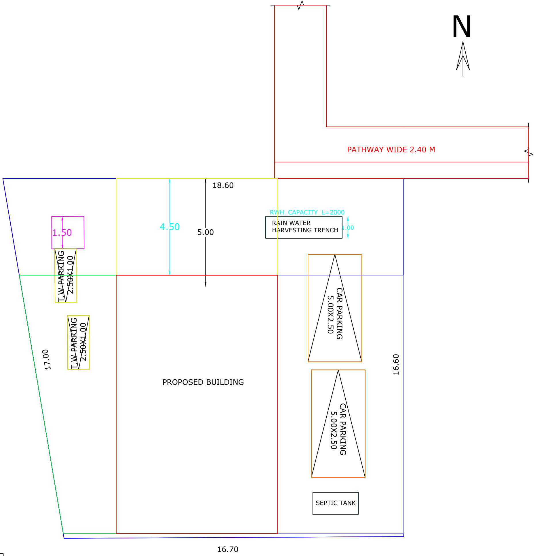
SITE PLAN
