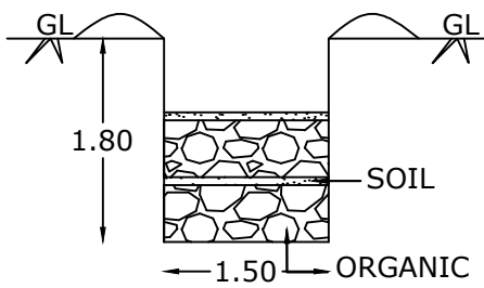
COMPOST PIT
