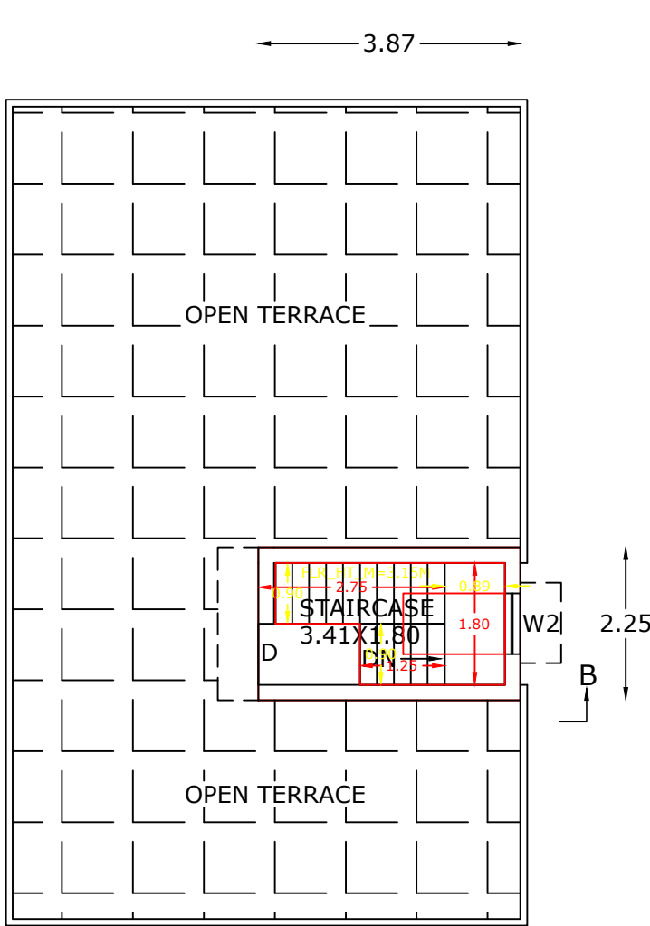
HEAD ROOM PLAN
