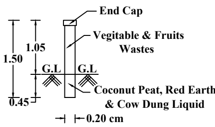
PIPE COMPOSTER
