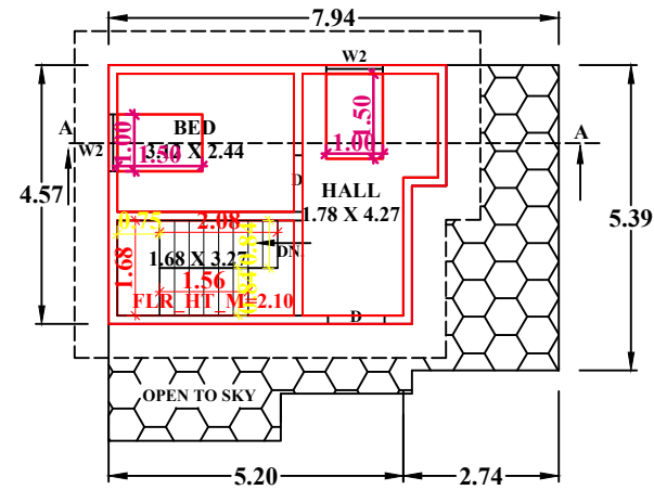
PLAN (FIRST FLOOR)
