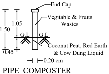
PIPE COMPOSTER
