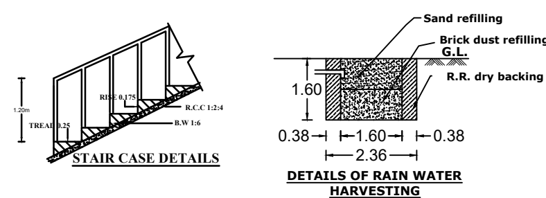
DETAILS OF RAIN WATER HARVESTING
