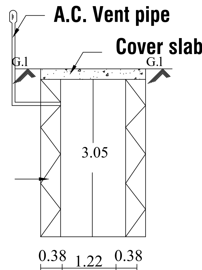
Soakpit section
