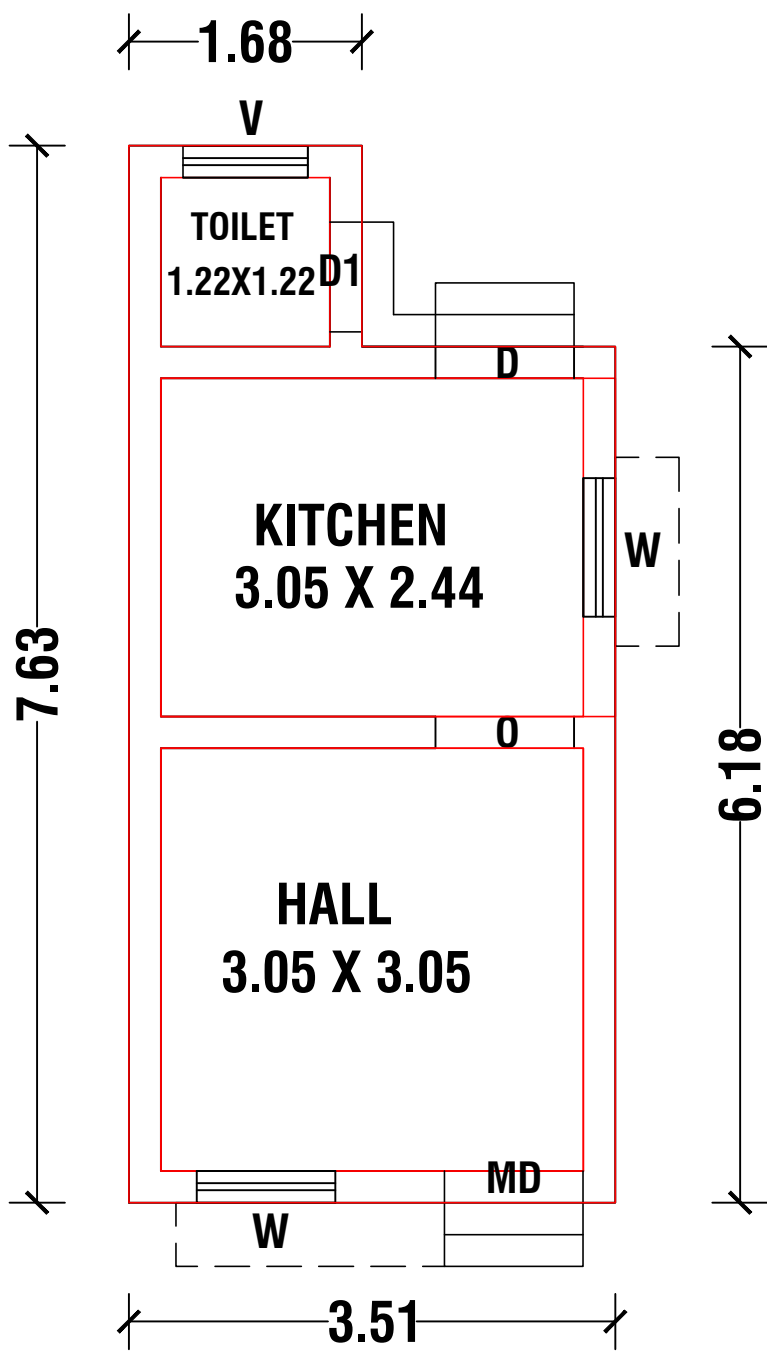
GROUND FLOOR PLAN SCALE 1:100 ALL DIMS ARE IN METRE
