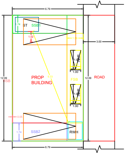
SITE PLAN [1:100]
