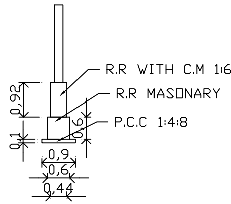
FOUNDATION
