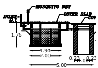
SECTION OF SEPT
