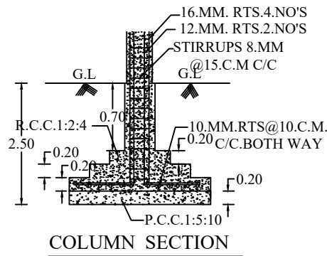
COLUMN SECTION
