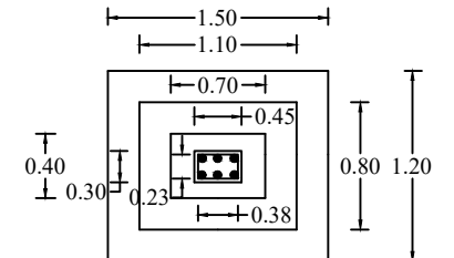
COLUMN PLAN (0.38x0.23 Size)
