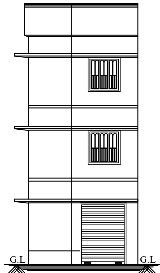
FRONT ELEVATION
