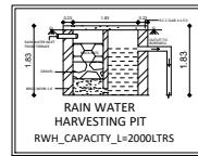
SECTION AB
