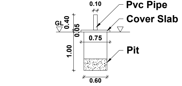
SOLID WASTE COMPOST PIT
