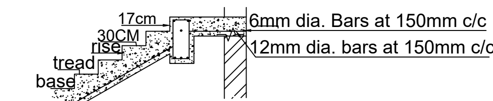
SECTION OF STAIRCASE
