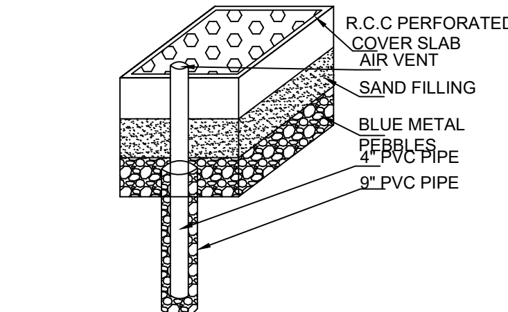
PERCOLATION BORE PIT
