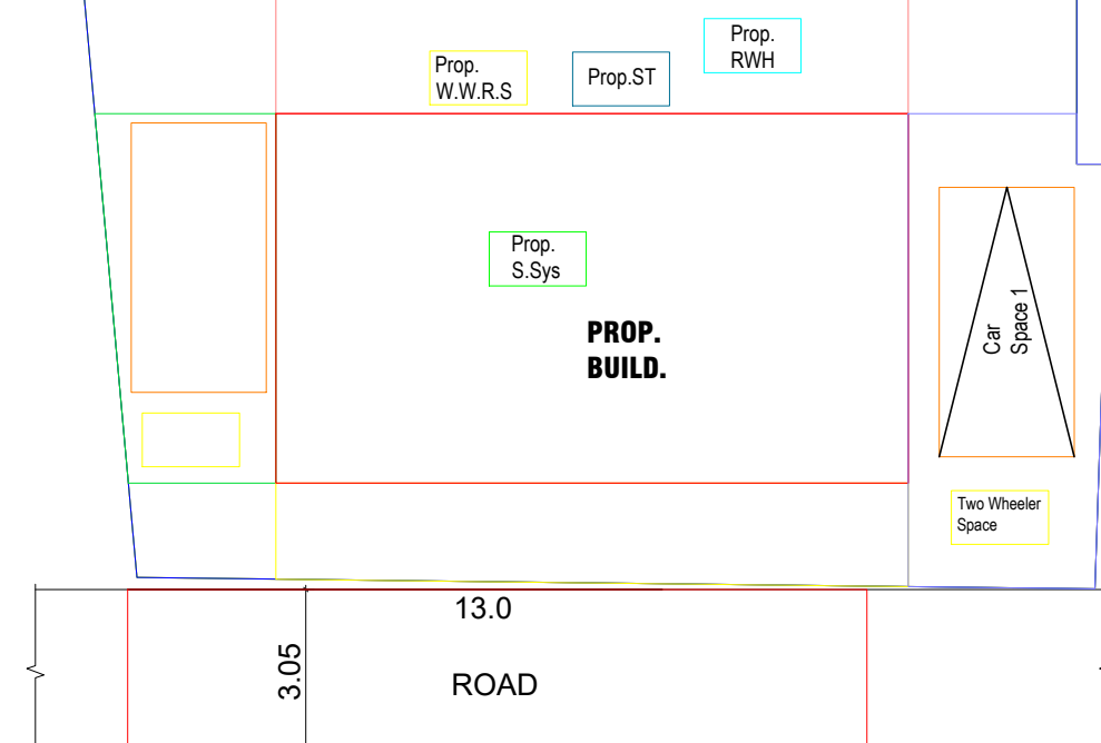
SITE PLAN SCALE:1:100.
