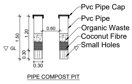
PIPE COMPOST PIT
