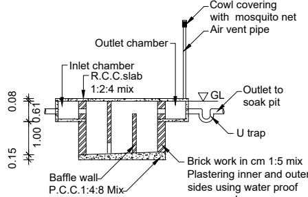
SECTION UV
