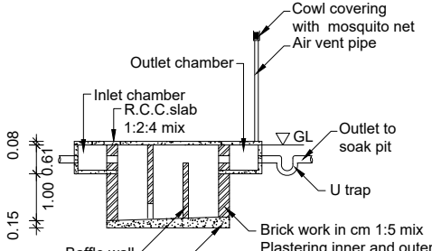
SECTION UV
