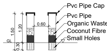
PIPE COMPOST PIT
