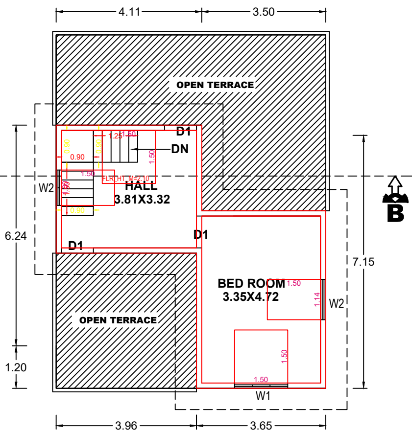
FIRST FLOOR
