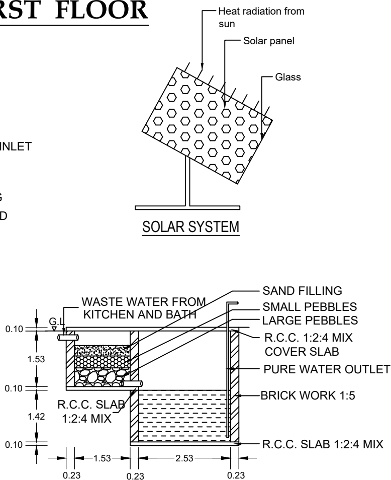
WASTE WATER RECYCLING SYSTEM
