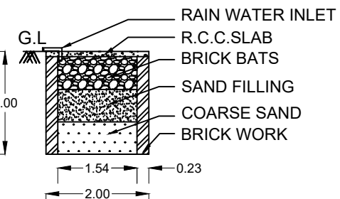
SECTION EF PLAN RAIN WATER PIT
