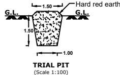
TRIAL PIT (Scale 1:100)
