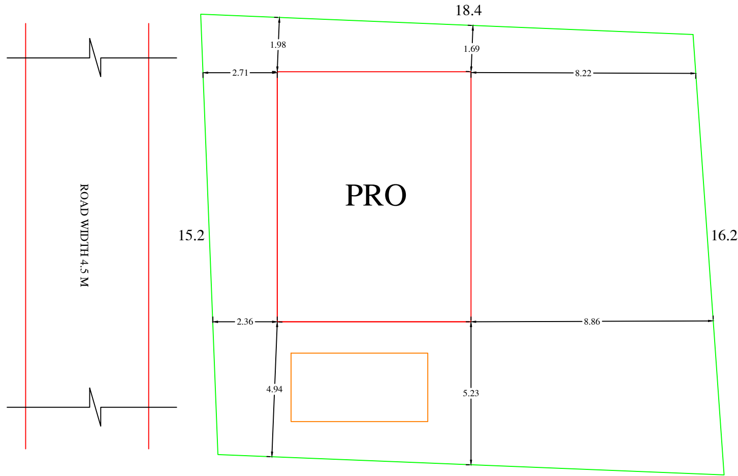
SITE PLAN
