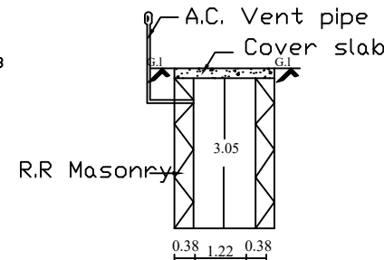
FOUNDATION
