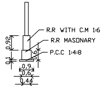
FOUNDATION
