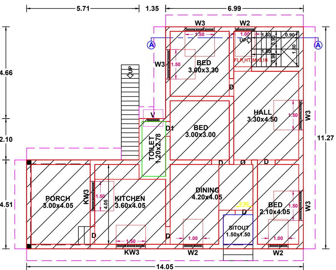
GROUND FLOOR PLAN HOUSE -1
