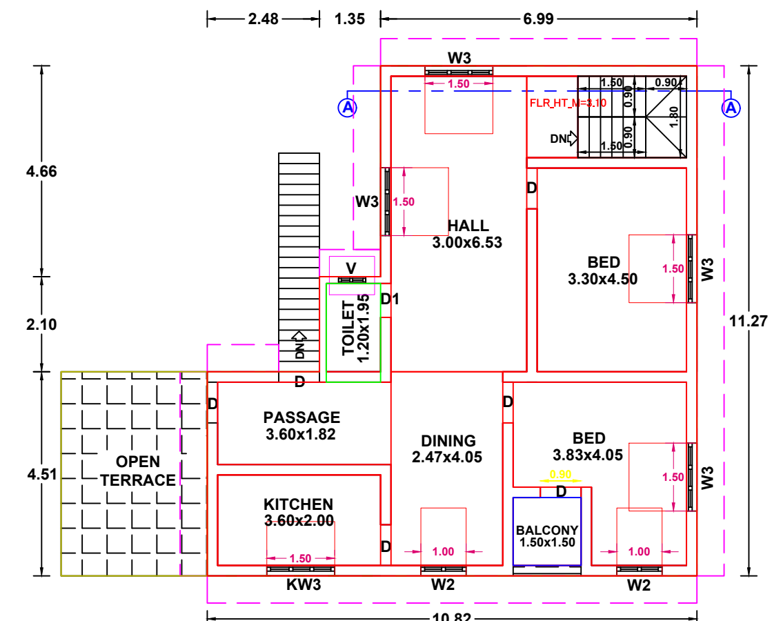
FIRST FLOOR PLAN HOUSE -2
