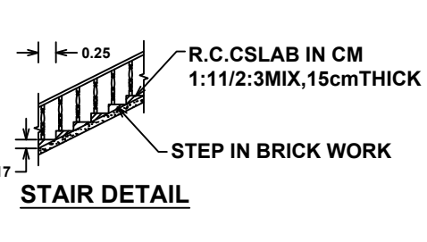
STAIR DETAIL
