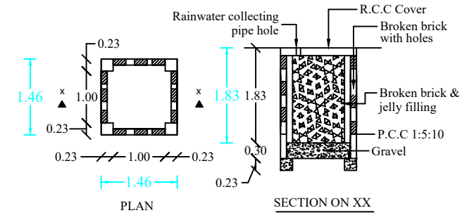
RAIN WATER HARVEST WELL RWH CAPACITY L=6642LTRS
