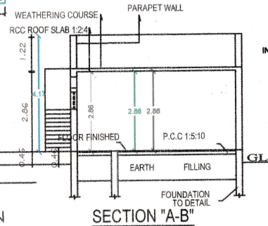
SECTION "A-B"
