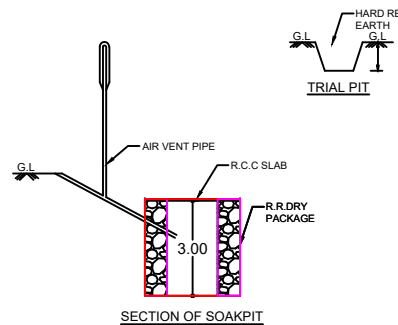
SECTION OF SOAKPIT
