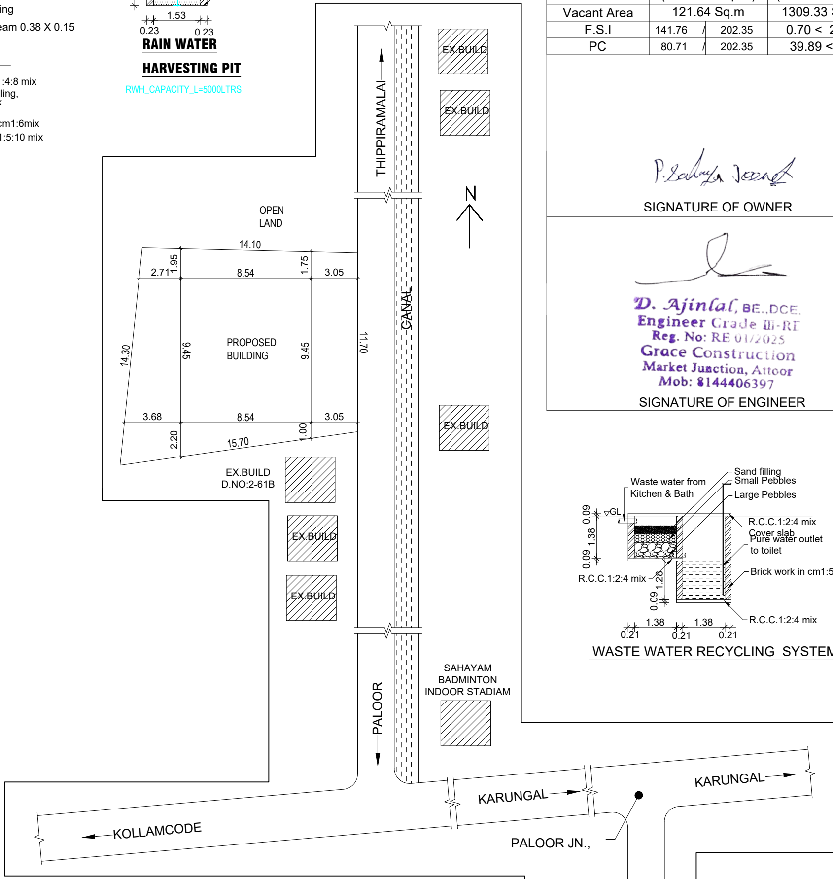
KEY PLAN
