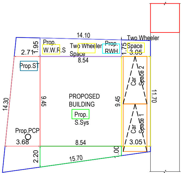
SITE PLAN
