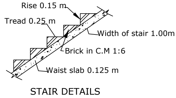
STAIR DETAILS
