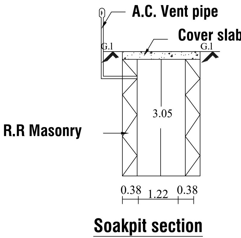
Soakpit section
