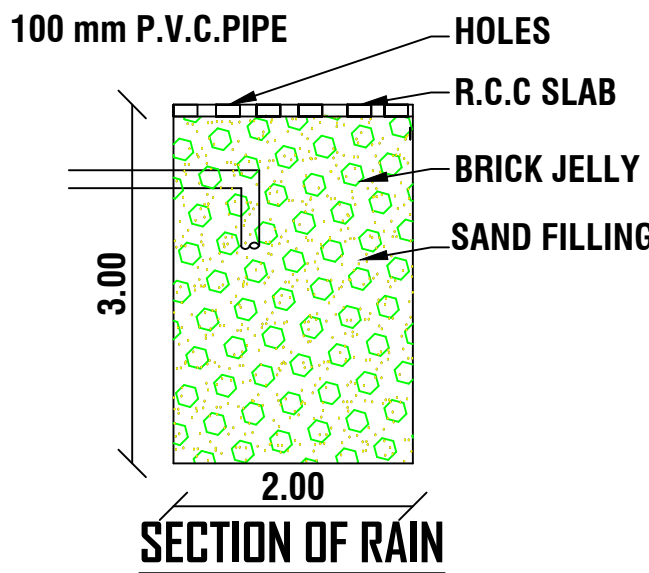
SECTION OF RAIN
