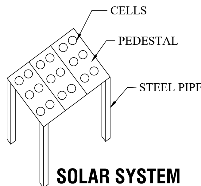
SOLAR SYSTEM
