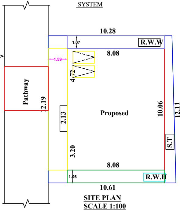
RAIN WATER SYSTEM
