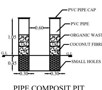
PIPE COMPOSIT PIT
