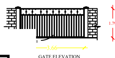
GATE ELEVATION
