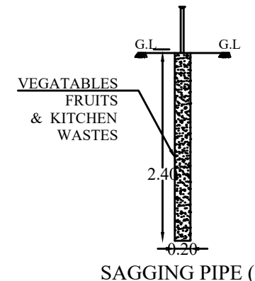
SAGGING PIPE (SP)
