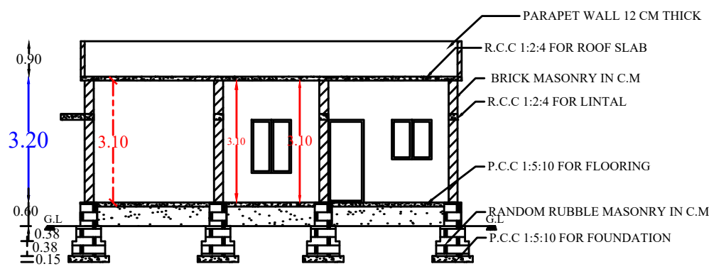
SECTION
