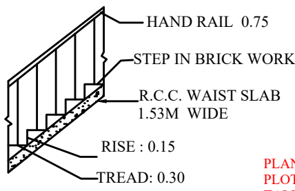
STAIR CASE SECTION
