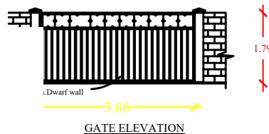
GATE ELEVATION
