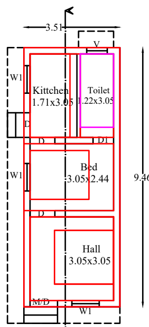
PLAN
