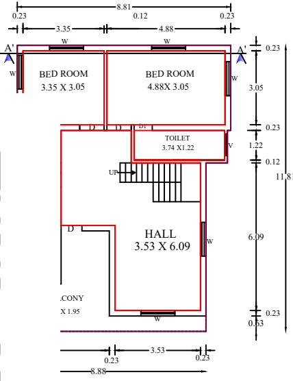
RST FLOOR
