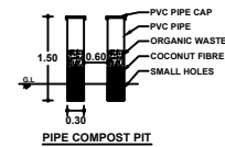
PIPE COMPOST PIT
